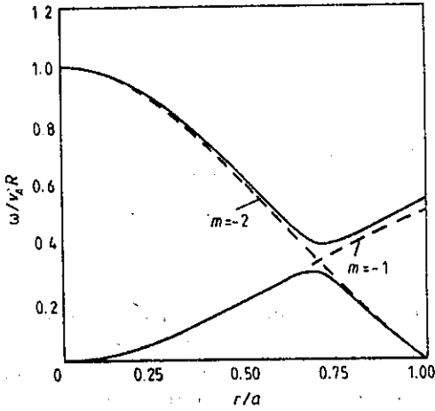
Figure 11.1 Toroidal Alfvén eigenmode spectrum in a tokamak.
