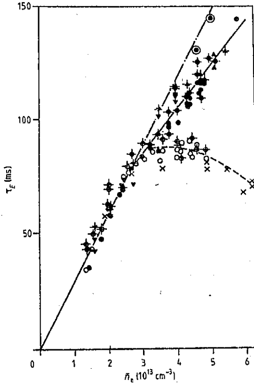
Figure 8.9 Improved ohmic confinement mode in ASDEX: the broken curve corresponds to the saturation mode; dots and circles—two different roc modes [88].
