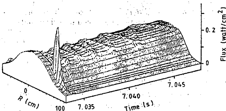
Figure 5.5 Soft x-ray (vertical camera, 140 \mu\text{m} thick Be filter) around the time of pellet injection showing the initial peak from ablation and the subsequent 'snake' oscillations [37].
