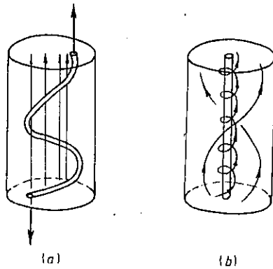
Figure 3.8 When the helical conductive filament (a) is stretched vertically the magnetic field lines become helical (b).
