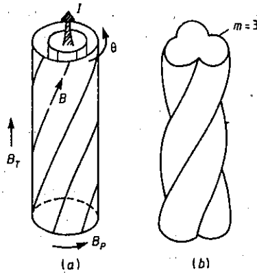
Figure 5.1 Helical perturbation of the tokamak plasma considered as a cylindrical column of length 2R with identical ends: (a) initial start; (b) perturbation of the m = 3 mode.
