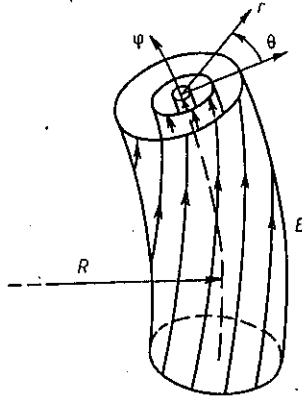
Figure 3.7 Magnetic field lines and coordinates r , \theta and \phi for a tokamak with a circularly-shaped plasma.
