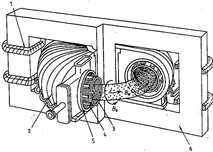
Figure 3.4 Schematic diagram of a tokamak: 1—primary transformer circuit; 2—toroidal field coils; 3—liner; 4—poloidal field coils; 5—copper shell; 6—iron transformer core.
