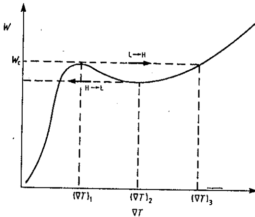
Figure 9.9 Thermal flux to the wall as a function of the edge plasma temperature gradient [117]. Depression of thermal conductivity is produced by turbulence suppression due to shear rotation of plasma [128].
