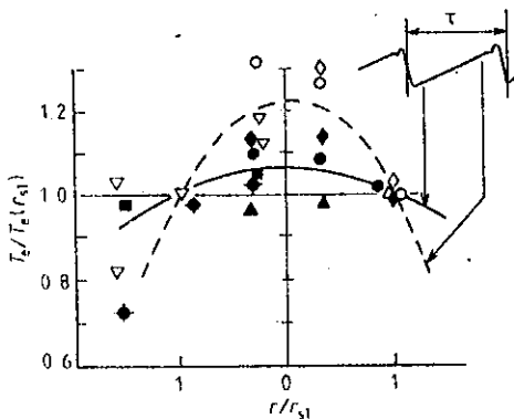
Figure 7.1 Electron-temperature-profile flattening at an internal disruption.
