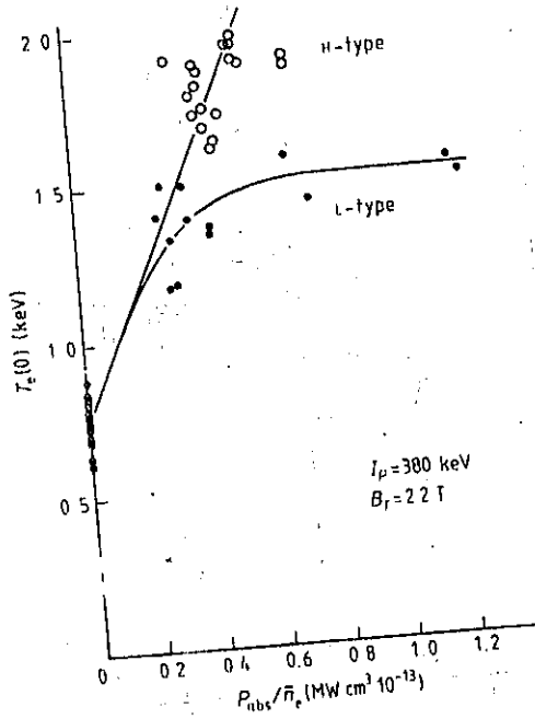
Figure 8.4 Electron temperature in L and H modes in ASDEX [17].
