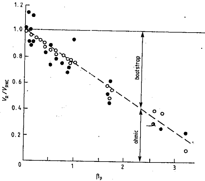
Figure 8.3 Bootstrap-current dependence on poloidal \beta_p [103].
