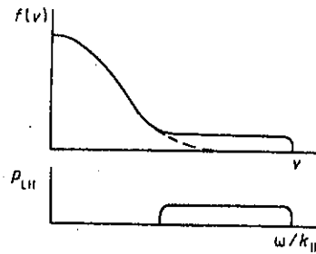
Figure 10.1 Electron distribution function modification by low-hybrid waves.
