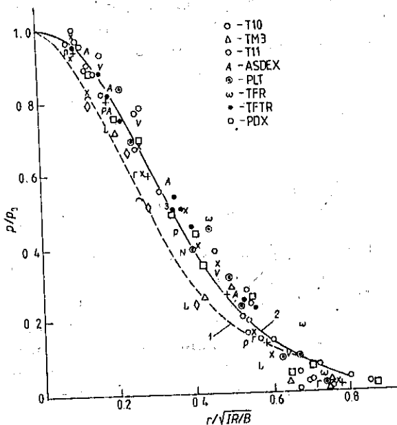
Figure 9.4 Comparison of the plasma pressure distribution profiles with the experimental data: 1— p = p_0(1 + \rho^2)^{-2} ; 2— p = p_0(1 + \rho^2)^{-6} .
