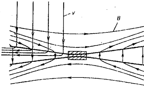
Figure 7.3 Plasma expulsion along the layer during reconnection.
