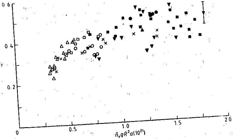
Figure 8.7 Saturation of \tau_E with density in the TFTR ohmic regime [108].
