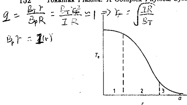
Figure 9.1 Three different plasma regions: 1—saw-tooth activity; 2—confinement region; 3—edge plasma.
