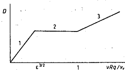
Figure 8.2 Schematic dependence of diffusion coefficient D and thermal diffusivity on the collisional frequency.
