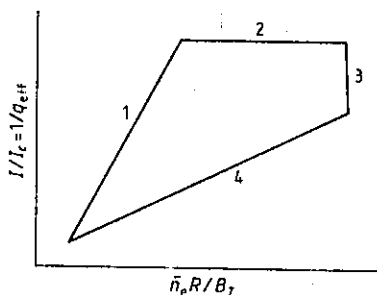
Figure 3.9 Hugill plot for tokamak plasma operation region: 1—run-away electron limit; 2—current limit; 3—Murakami density limit; 4—Hugill limit.
