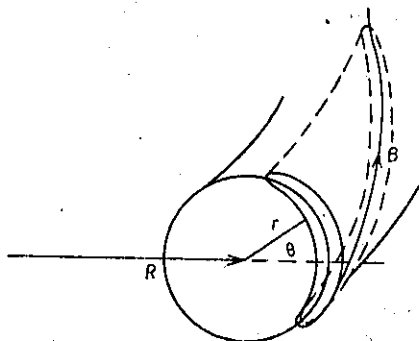
Figure 8.1 Trapped particle trajectories ('banana').
