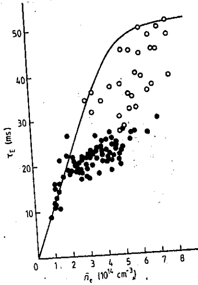
Figure 8.6 Confinement improvement in ALCATOR-C with pellet injection [17].
