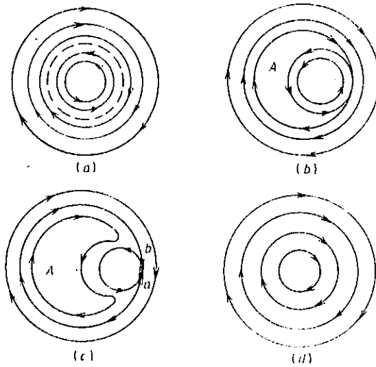
Figure 7.2 Process of reconnections on auxiliary transverse magnetic field B^* : (a) direction of magnetic lines relative to the surface with B^* = 0 ; (b) contact of surfaces with oppositely directed fields B^* ; (c) reconnection of the current layer ab due to finite plasma conductivity; (d) final result of reconnections: auxiliary magnetic field is unidirectional.
