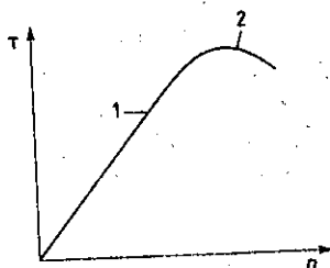
Figure 8.12 The best theoretical mode of confinement looks like a superposition of the superclassical confinement (1) and electron plus ion neoclassical confinements (2).
