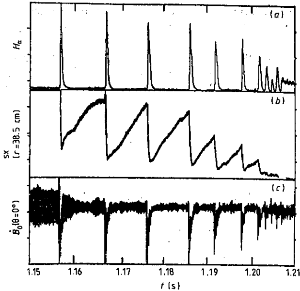
Figure 7.7 Oscillations in the ELM mode [87].
