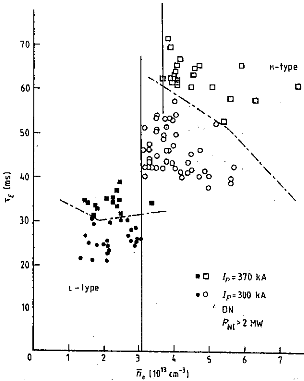
Figure 8.5 Density threshold for L-H transition in ASDEX [17].
