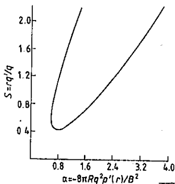
Figure 5.8 Schematic diagram for the ballooning instability region.
