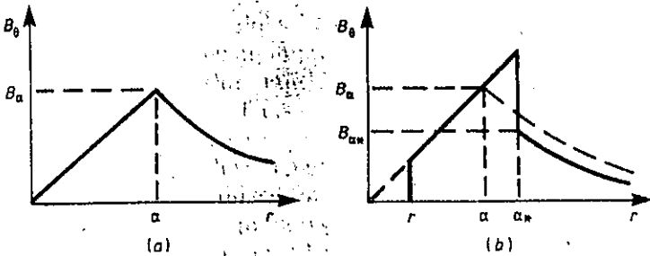
Figure 5.4 Poloidal magnetic field distribution in the initial state (a) and in the final state (b) with a single cylindrical bubble.
