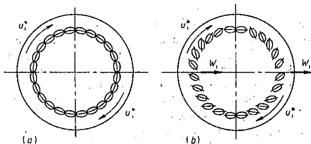
Figure 9.5 Magnetic island structures: (a) in the cylindrical plasma column; (b) toroidal variant of island structure which can be pumped by ions.
