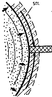
Figure 4.4 Scrape-off layer (sol).
