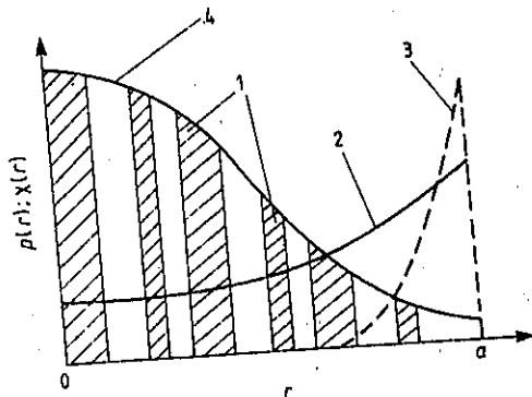
Figure 9.10 Schematic diagram of the plasma transport self-organization: 1—thermal flux produced by deviation from optimal profile; 2—bulk plasma transport; 3—transport at the plasma edge; 4—pressure profile.
