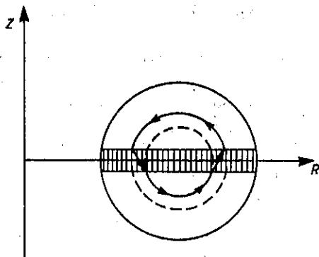
Figure 9.6 If the drift turbulence fills the hatched area and the phases of perturbations allow for ions to be shifted radially while crossing this area, then a single ion can transform some part of its energy into the energy of noise. This transformation is based on the conservation of azimuthal and magnetic momentum.
