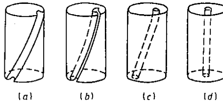
Figure 5.3 Non-linear kink instability and helical bubble injection into plasma.
