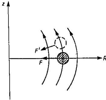
Figure 3.5 Equilibrium magnetic barrel-type field lines. When the plasma torus is shifted vertically the restoring force F' generates a vertical component directed towards the median plane.
