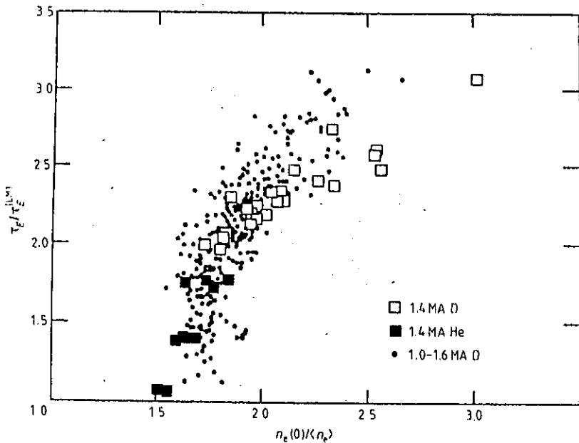
Figure 8.8 Plasma energy confinement improvement in TFTR as a result of density-profile peaking [139].
