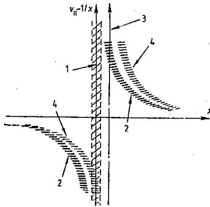
Figure 9.8 Contact between the plateaux of two neighbouring island chains in phase space: 1—rational surface and island chain (hatched area) of the first wave; 2—plateau on f_e(v_{||}) ; 3—second rational surface; 4—plateau formation due to the second island chain.
