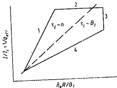
Figure 6.4 Boundary of the ALCATOR scaling on the Hugill diagram (broken line).
