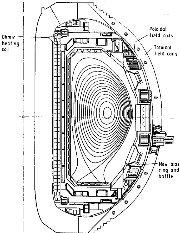
Figure 3.6 DIII-D tokamak elevation [147].
