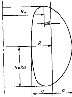
Figure 4.3 Parameters of D-shaped plasma: K = b/a —elongation.
